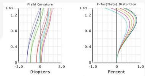
Distortion, Field Curvature & Astigmatism Analyzing & Optimization
