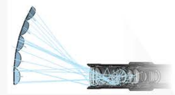
Stray Light Optical Design Analysis
